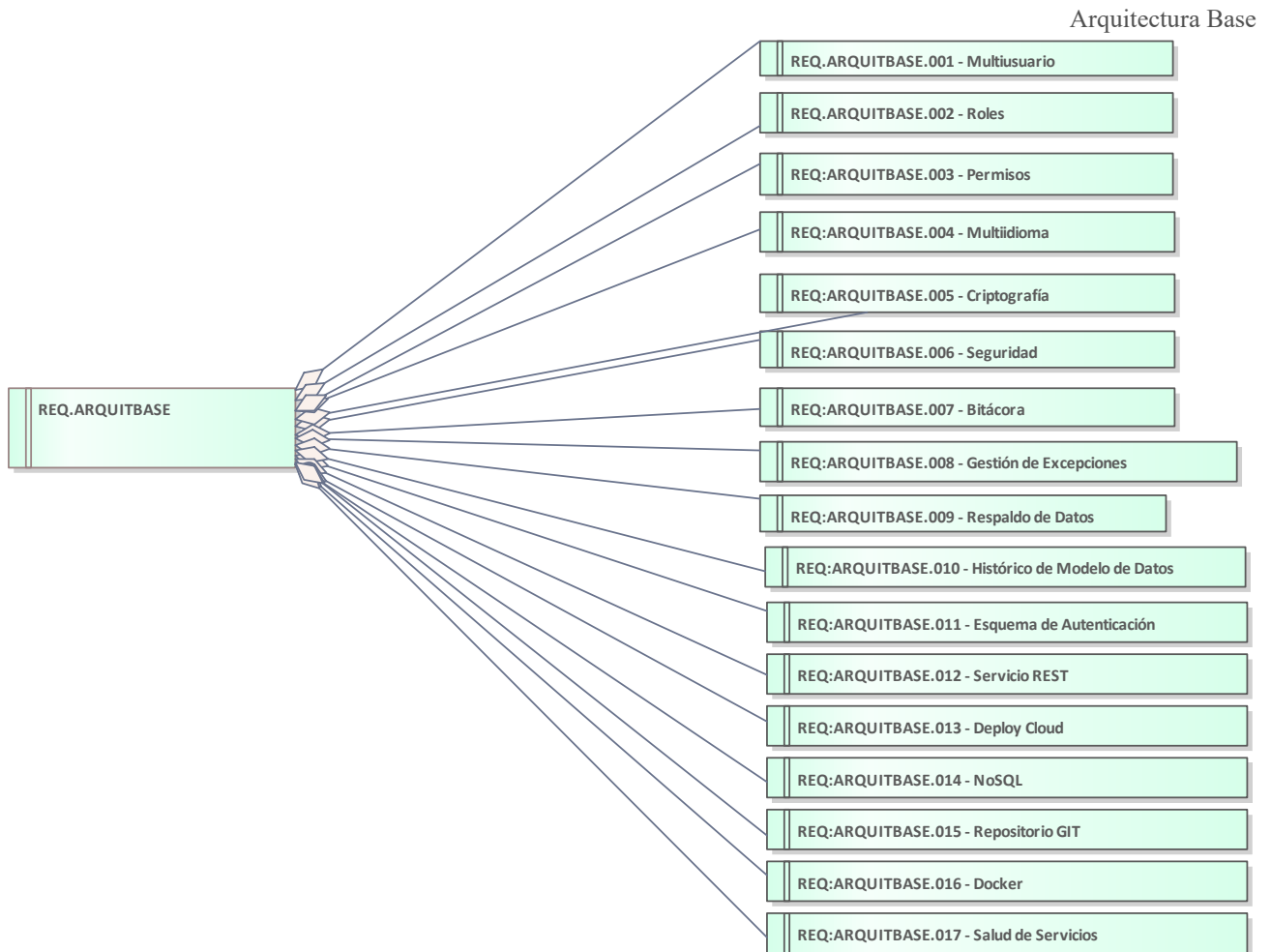
Figure 42: Arquitectura Base
