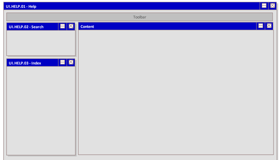
Figure 131: Help System
