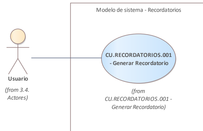
Figure 56: Recordatorios
