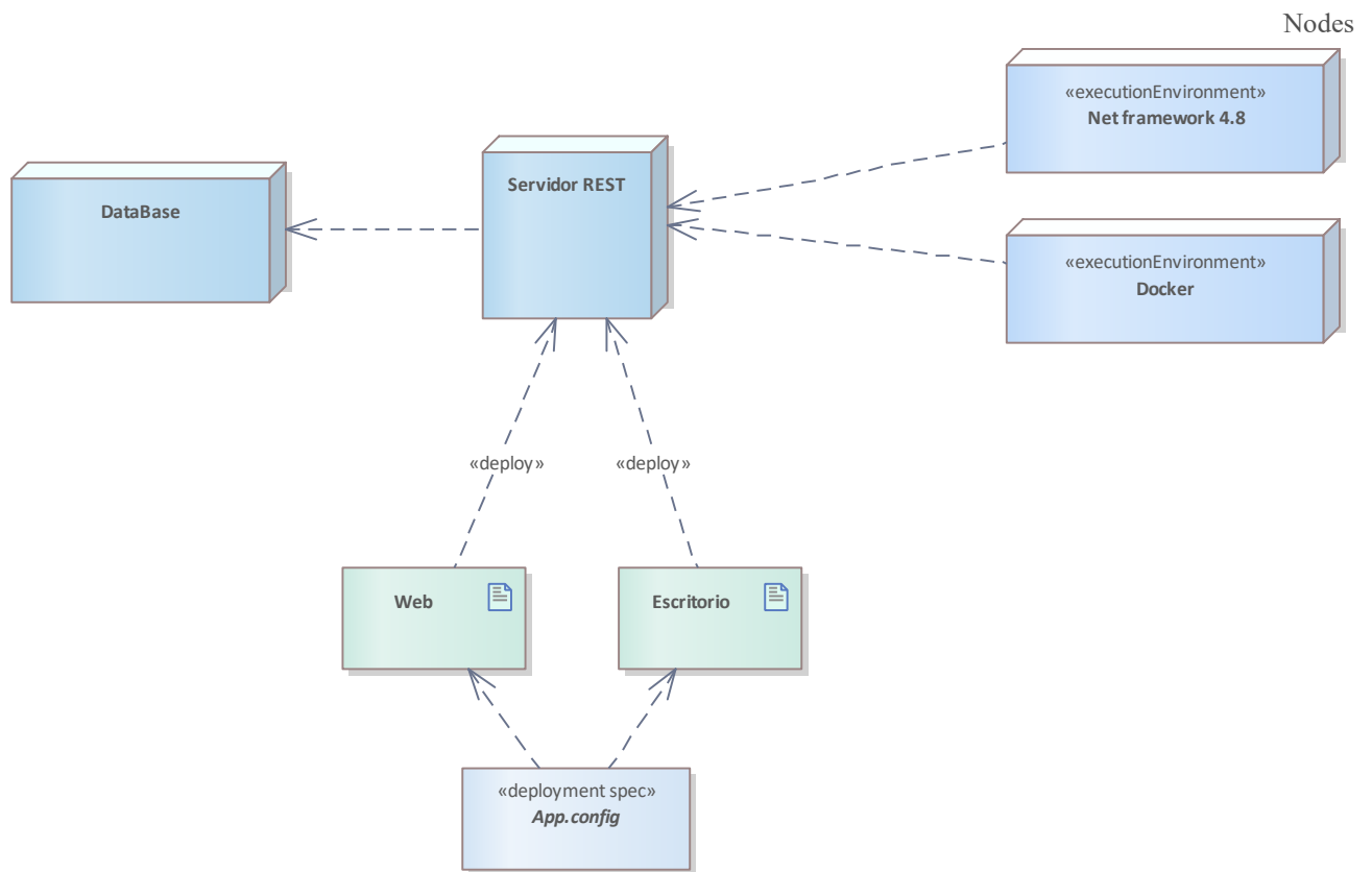
Figure 127: Nodes
