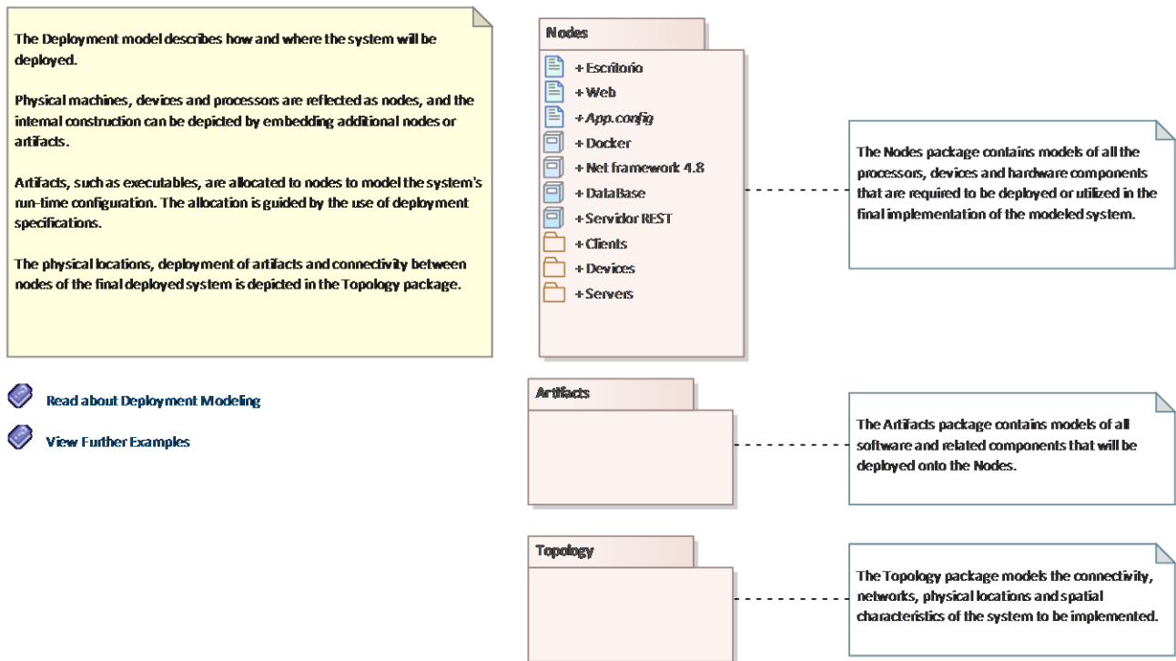
Figure 126: Deployment Model
